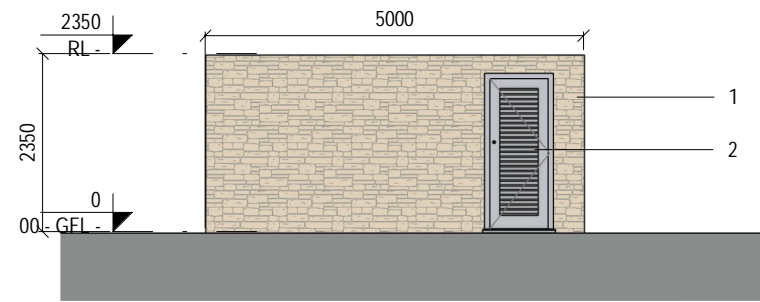
2 Front Elevation 1 : 100
