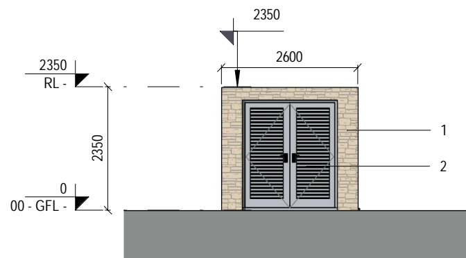
6 Side Elevation B 1 : 100
