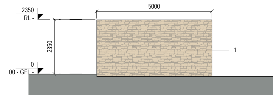
7 Rear Elevation 1 : 100
